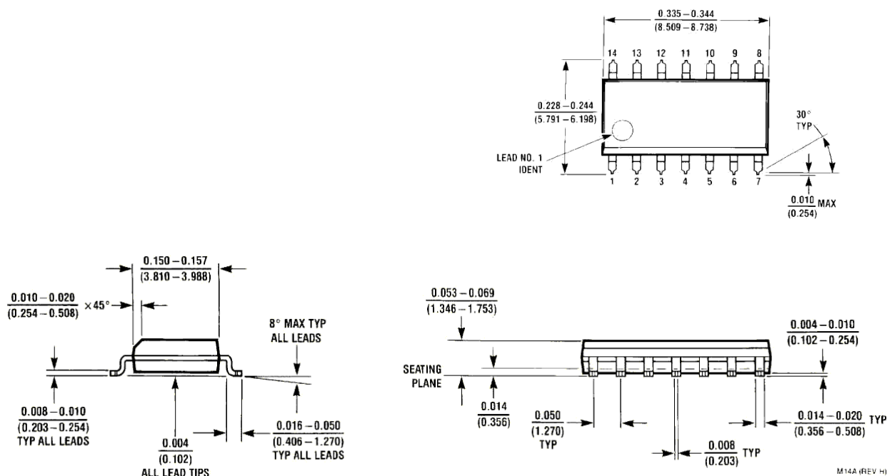
S.O. Package (M) Order Number LM339AM, LM339AMX, LM339M, LM339MX, LM2901M or LM2901MX NS Package Number M14A
