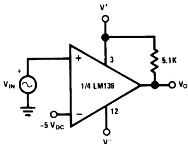
Comparator with a Negative Reference
