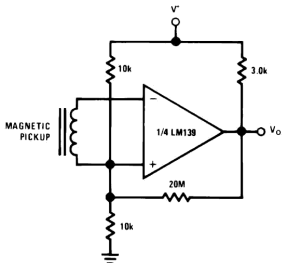
Transducer Amplifier
